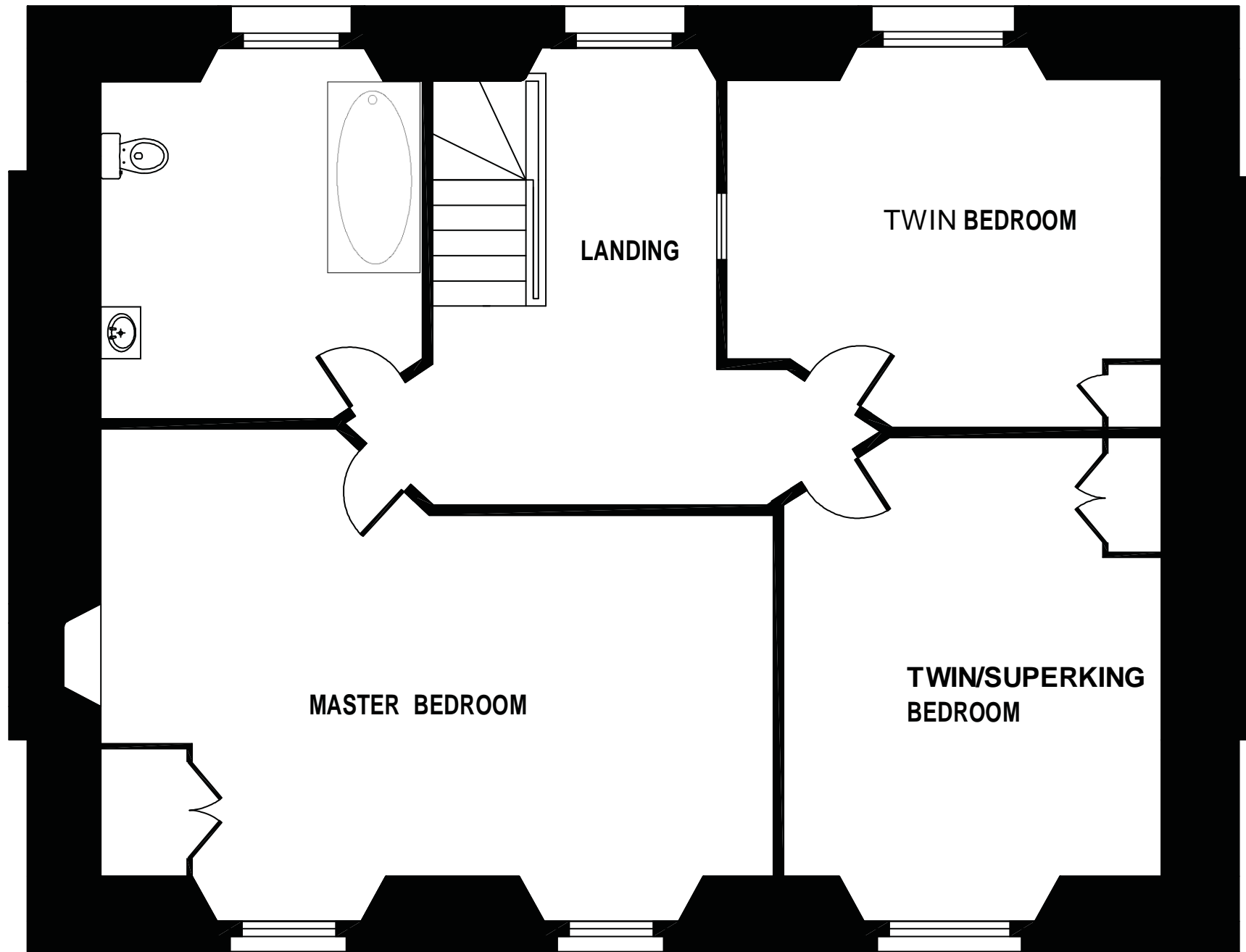
FIRST FLOOR
